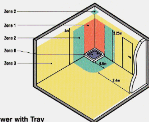
Shower without Tray but with permanently fixed partition - fixed water outlet not demountable
